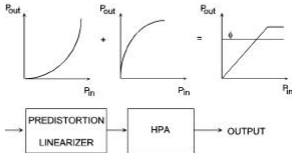
Figure 1. Predistortion linearization attempts to create an ideal limiter transfer characteristic
