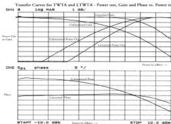
Figure 3. Linearized TWTA Transfer Response
