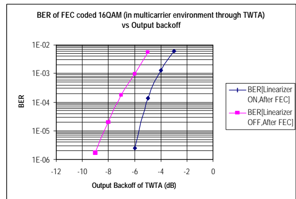
Figure 5. BER of Rate 3/4 convolutional FEC Data
