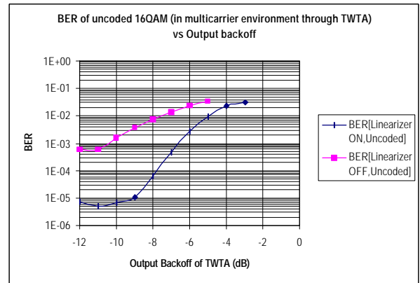
Figure 4. BER of Uncoded Data
