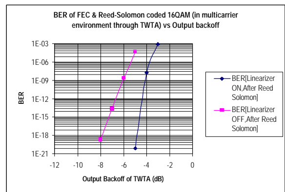
Figure 6. BER of FEC + RS Coded data
